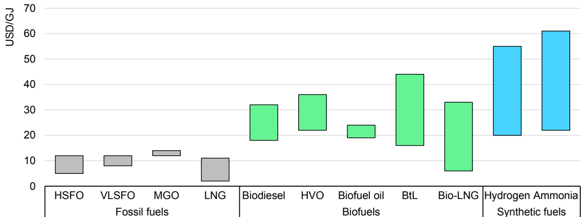
Figure 8.13 Indicative shipping fuel cost ranges
