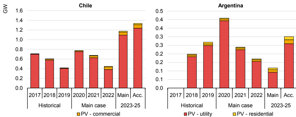
Figure 3.21 Chile and Argentina annual PV capacity additions 2017-22 and average annual additions 2023-25
