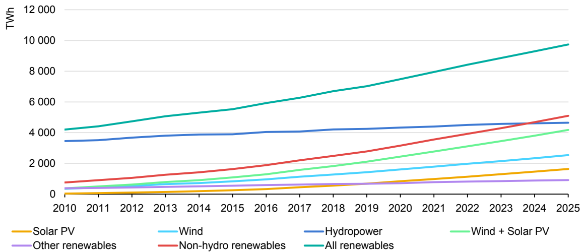
Figure 2.5 Renewable electricity generation by technology, 2010-25
