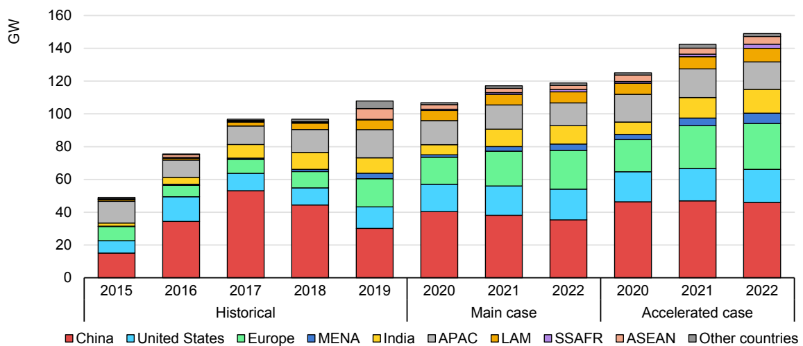
Figure 3.2 Solar PV net capacity additions by country/region
