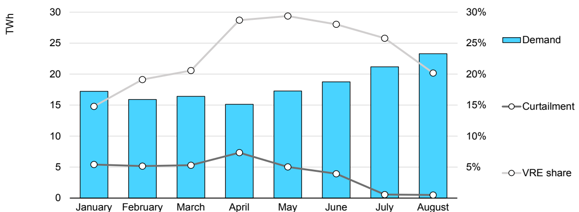
Figure 8.8 California demand, curtailment and VRE shares, 2020
