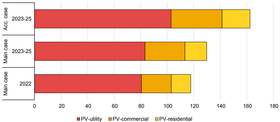
Figure 3.3 Average global annual capacity additions in main and accelerated cases, 2023-25
